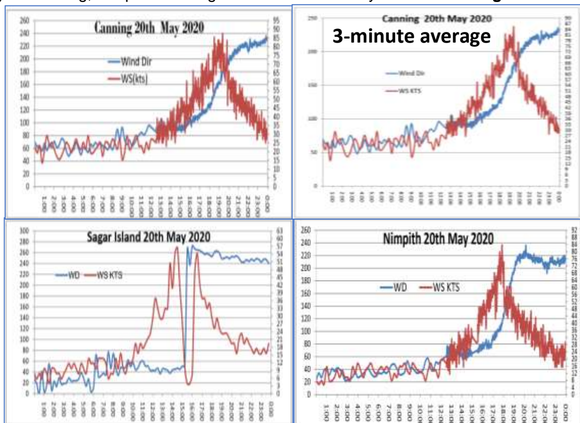
Fig.6: AWS data from Canning, Sagar Island & Nimpith on 20 th May 2020
