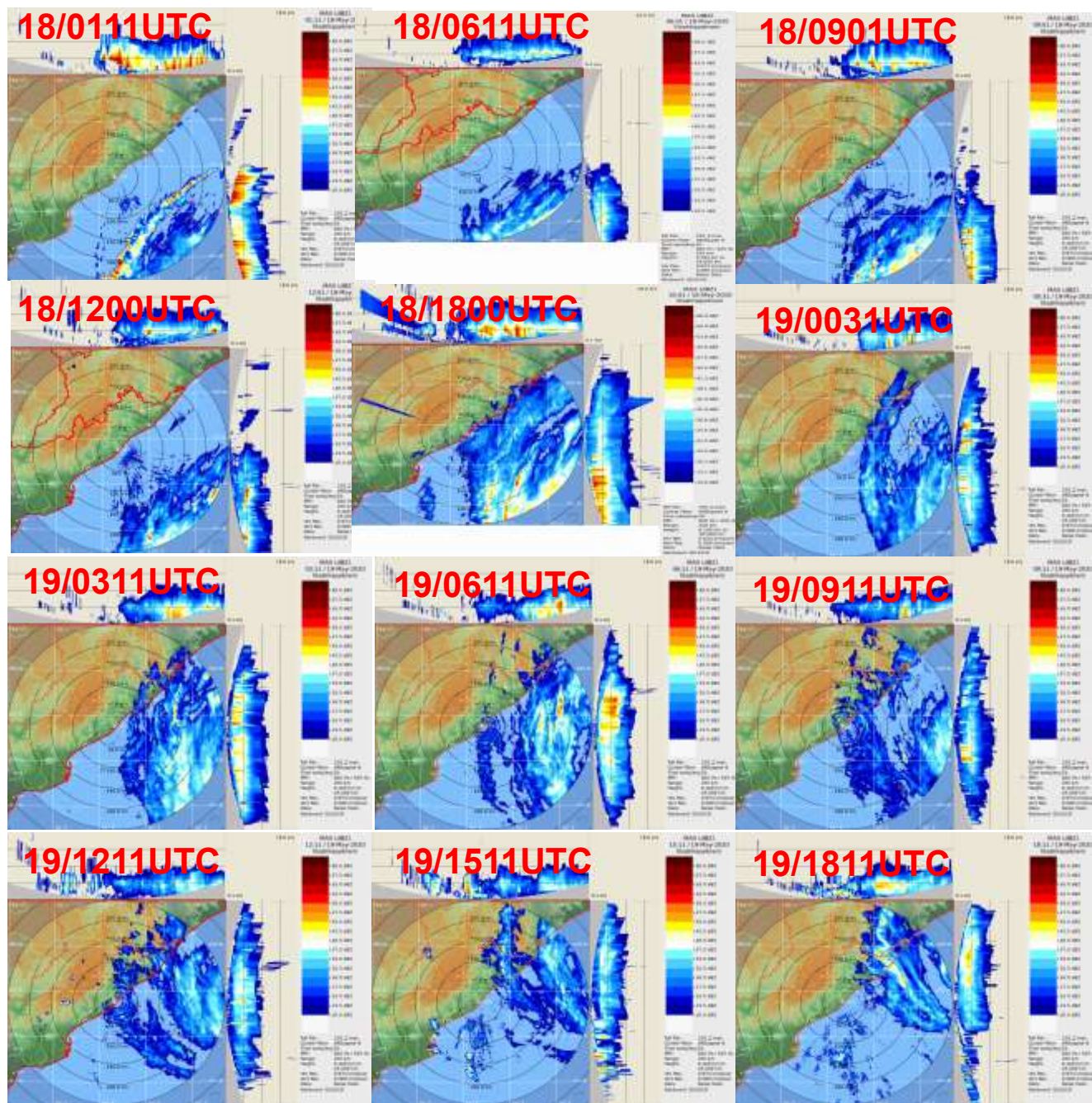
Fig. 8: Typical Radar Max dBZ imageries from DWR Visakhapatnam during 18-19 May, 2020
