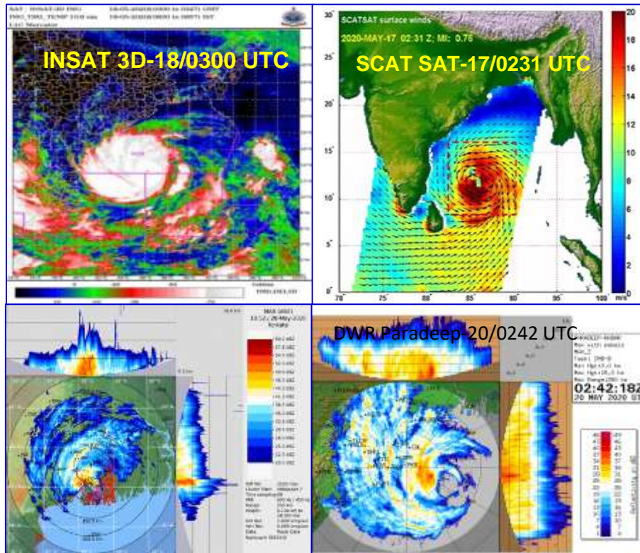
Fig.4: Typical satellite imageries for SuCS Amphan over the Bay of Bengal and Radar imageries from DWR Kolkata & Paradip
