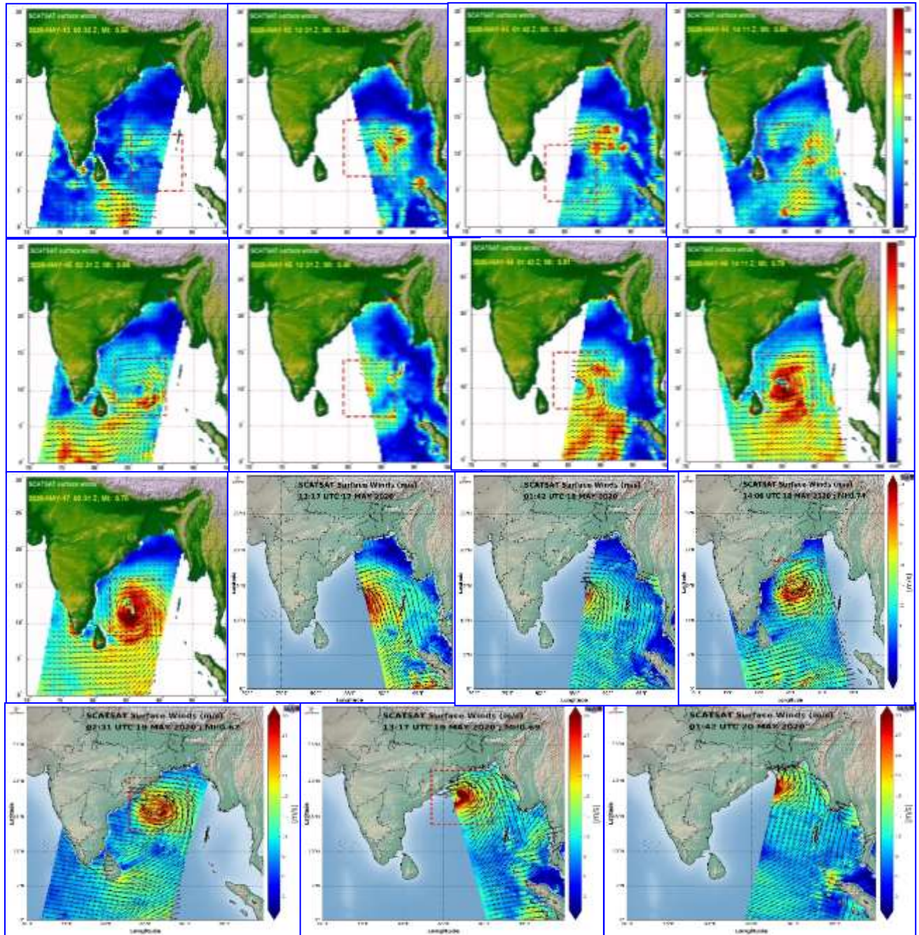
Fig. 6: SCAT SAT imageries during life cycle of SuCS AMPHAN (13-20 May, 2020)
