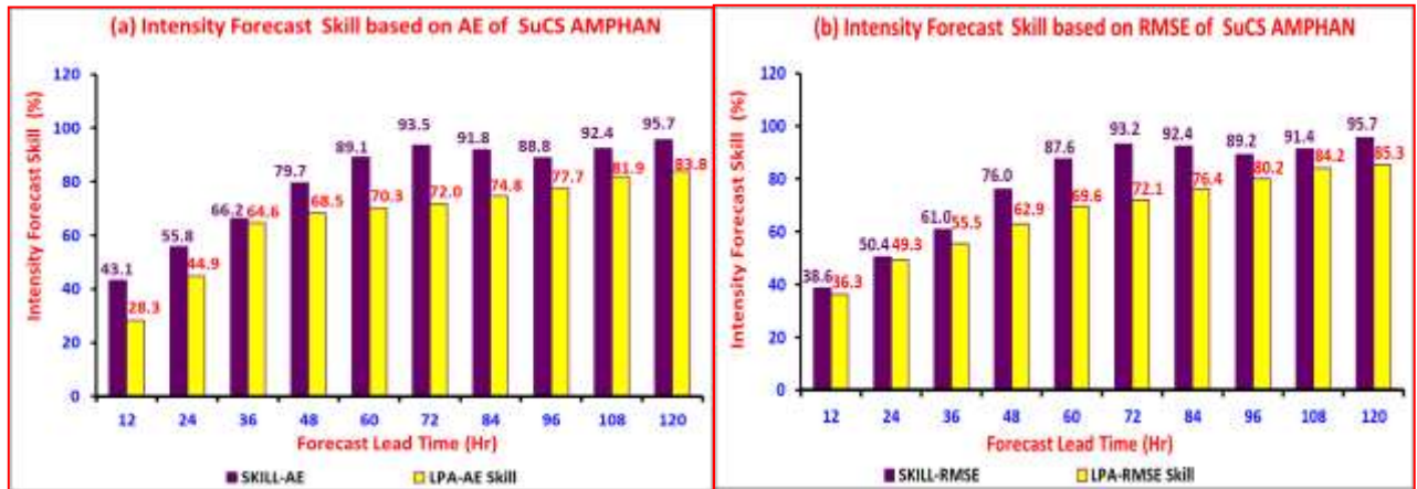
Fig. 12: Skill (%) in intensity forecast based on (a) Absolute errors (AE) and (b) Root Mean Square errors (RMSE) of SUCS AMPHAN as compared to long period average (2015-19)
