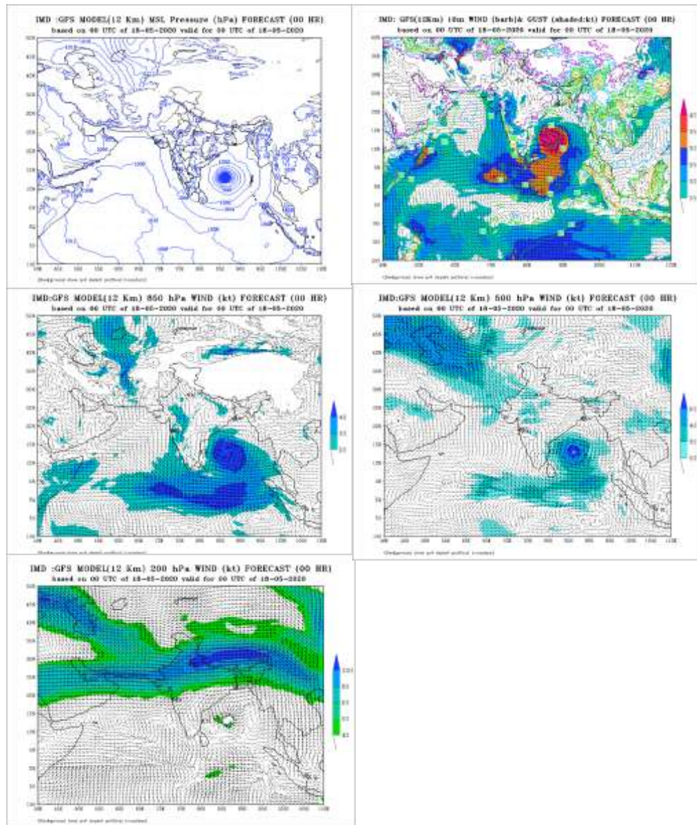
Fig. 14 (f): IMD GFS (T574) mean sea level pressure (MSLP), winds at 10m, 850, 500 and 200 hPa levels based on 0000 UTC of 18 th May,2020
