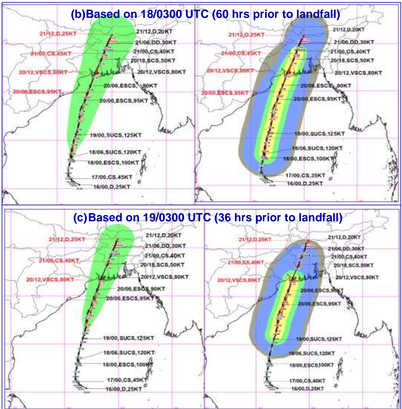
Fig.8(b) &(c): Observed and forecast track alongwith cone of uncertainty and quadrant wind distribution based on (b) 0300 UTC of 18 th May (60 hours prior to landfall) and (c) 0300 UTC of 19 th May (36 hours prior to landfall) of SuCS AMPHAN indicating accuracy in landfall, track & intensity predictions
