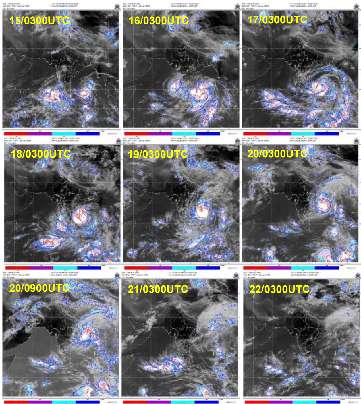
Fig. 5: INSAT-3D Cloud Top Brightness Temperature (CTBT) imageries during life cycle of SuCS AMPHAN (15-22 May, 2020)
