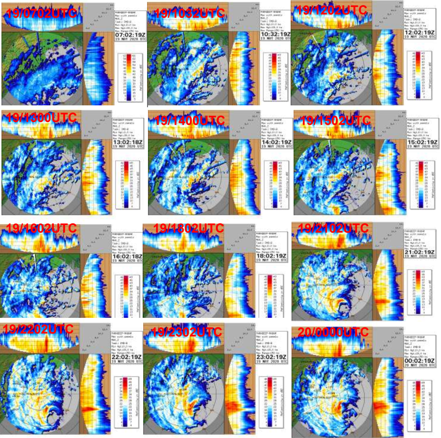
Fig. 10 a: Typical Radar Max Z imageries of DWR Paradeep during during 19-20 May, 2020
