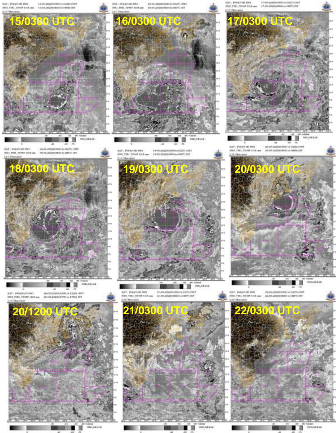
Fig. 2: INSAT-3D BD imageries during life cycle of SuCS AMPHAN (15-22 May, 2020)
