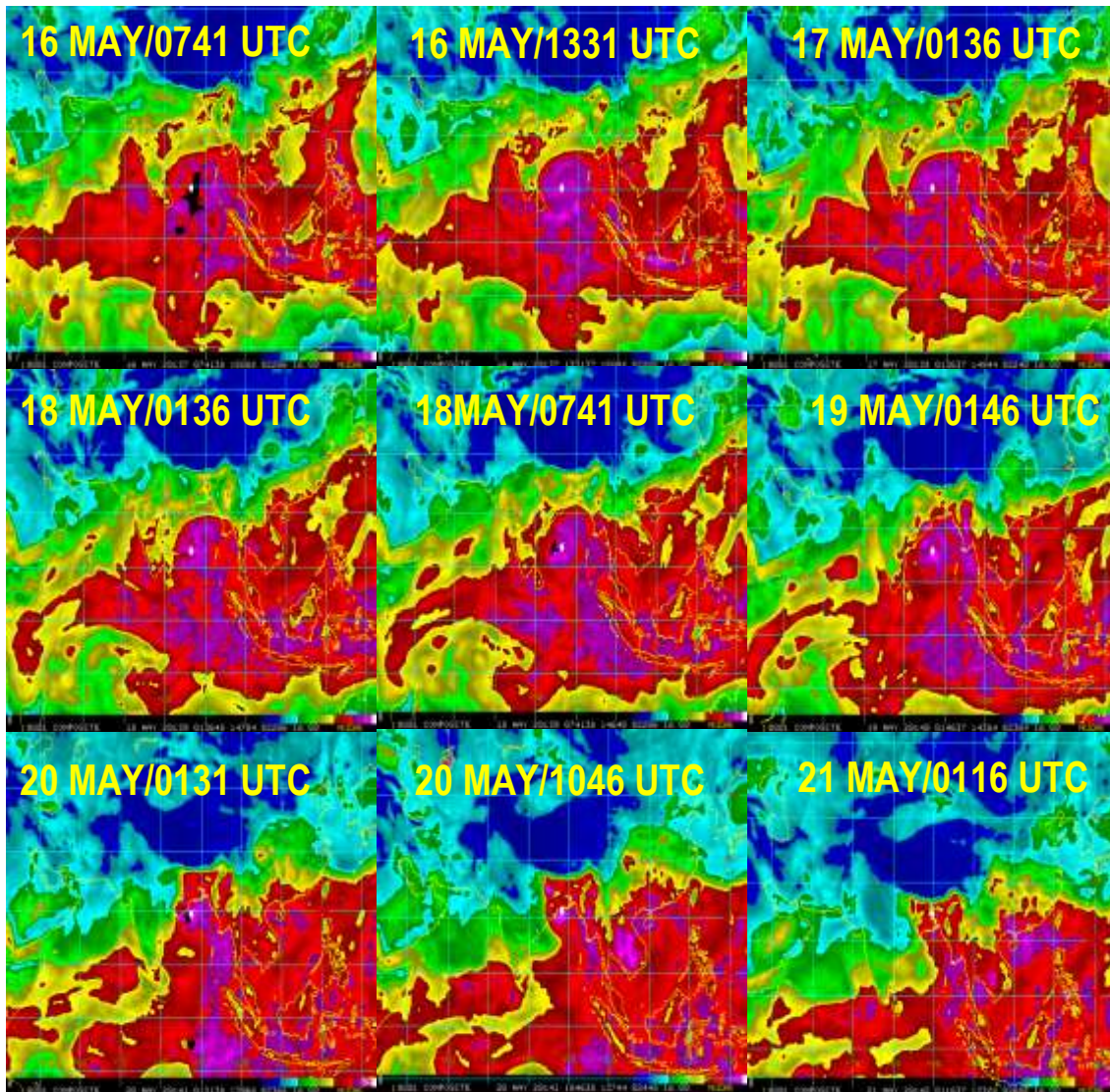
Fig. 13: Typical total precipitable water imageries during life cycle of SuCS Amphan (16 th -21 st May, 2020).
