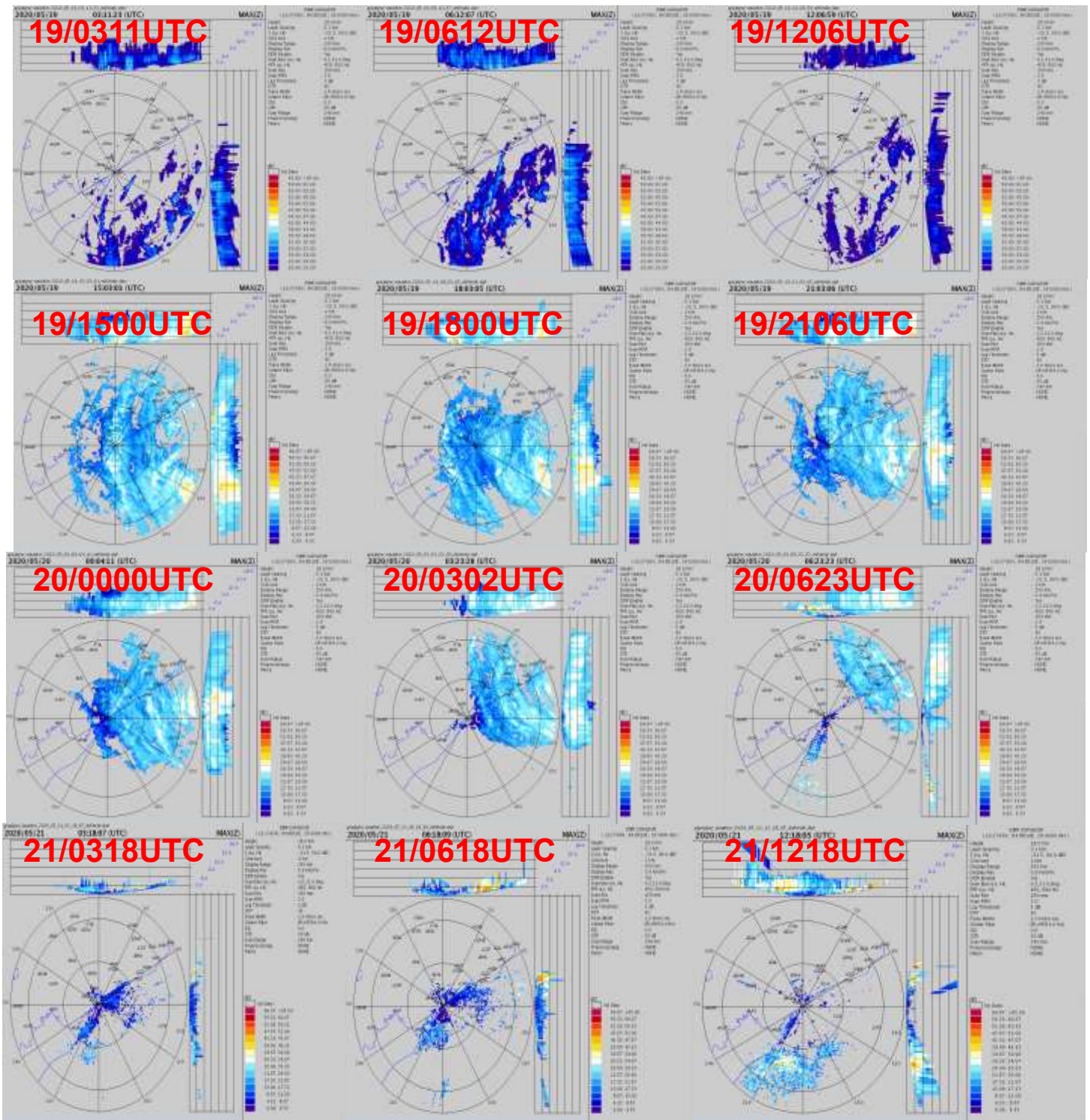
Fig. 9: Typical Radar Max Z imageries from DWR Gopalpur during during 19-21 May, 2020
