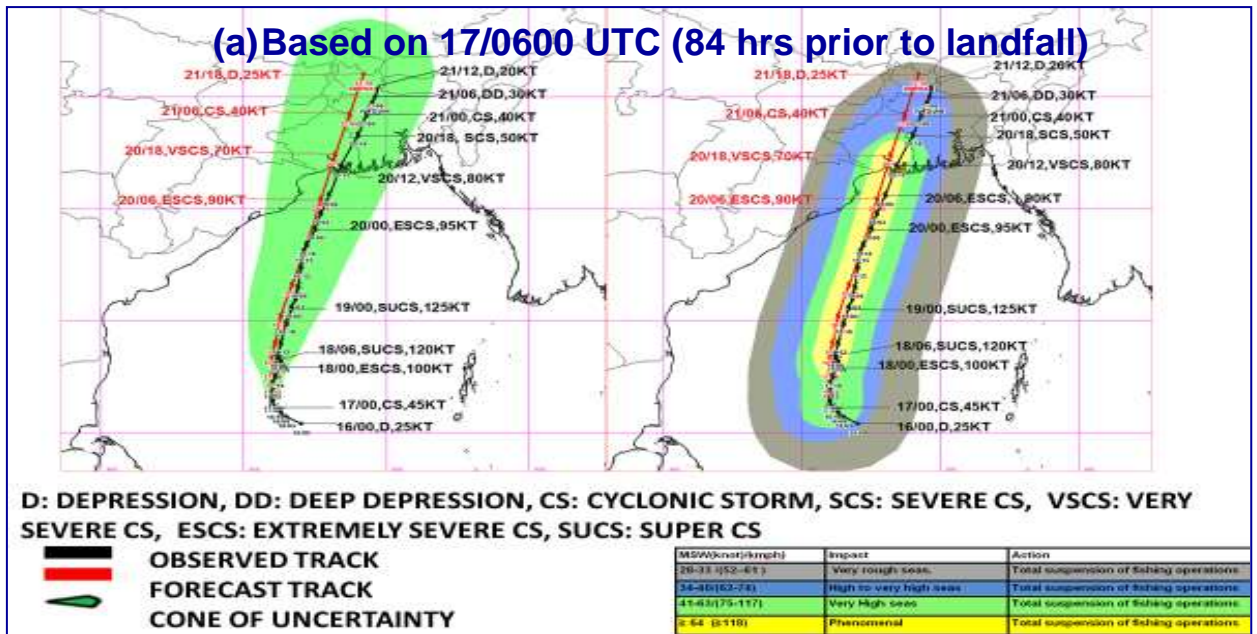
Fig.8(a): Observed and forecast track along with cone of uncertainty and quadrant wind distribution based on 0600 UTC of 17 th May (84 hrs prior to landfall) of SuCS AMPHAN indicating accuracy in landfall, track & intensity predictions
