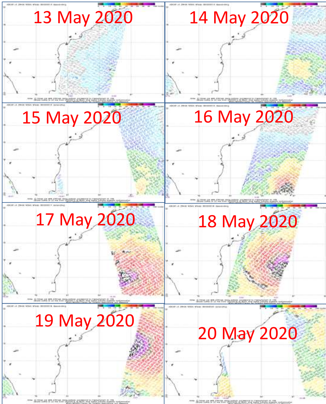
Fig. 7: ASCAT imageries during life cycle of SuCS AMPHAN (13-20 May, 2020)
