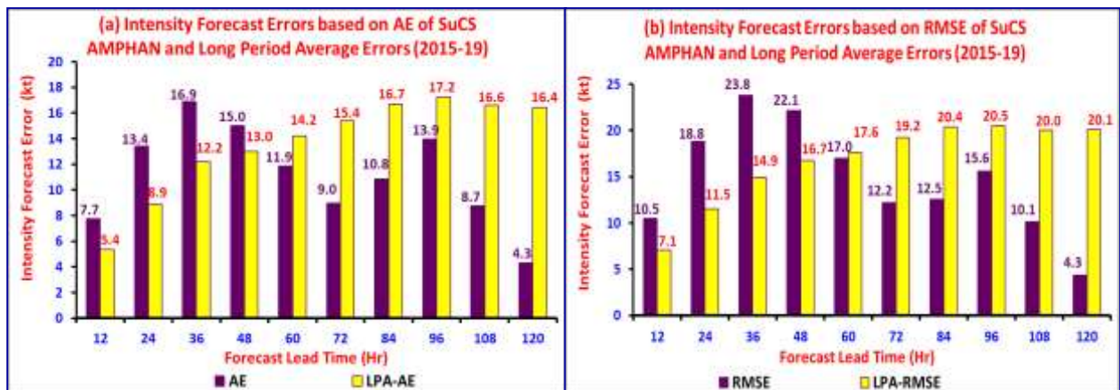
Fig. 11: Absolute errors (AE) and Root Mean Square errors (RMSE) in intensity forecast (winds in knots) of SUCS AMPHAN as compared to long period average (2015-19)
