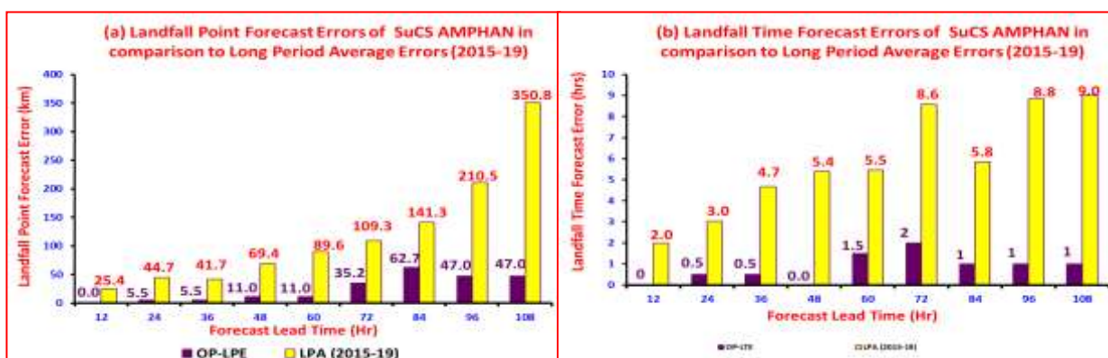
Fig. 9: Landfall (a) point and (b) time forecast errors of SuCS AMPHAN as compared to long period average (2015-19)
