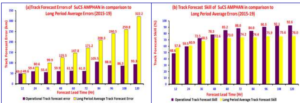
Fig. 10(a) & (b): Track forecast errors and skill of SUCS AMPHAN as compared to long period average (2015-19)
