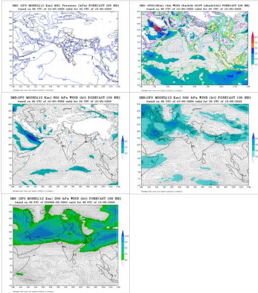
Fig. 14 (a): IMD GFS (T574) mean sea level pressure (MSLP), winds at 10m, 850, 500 and 200 hPa levels based on 0000 UTC of 13 th May,2020
