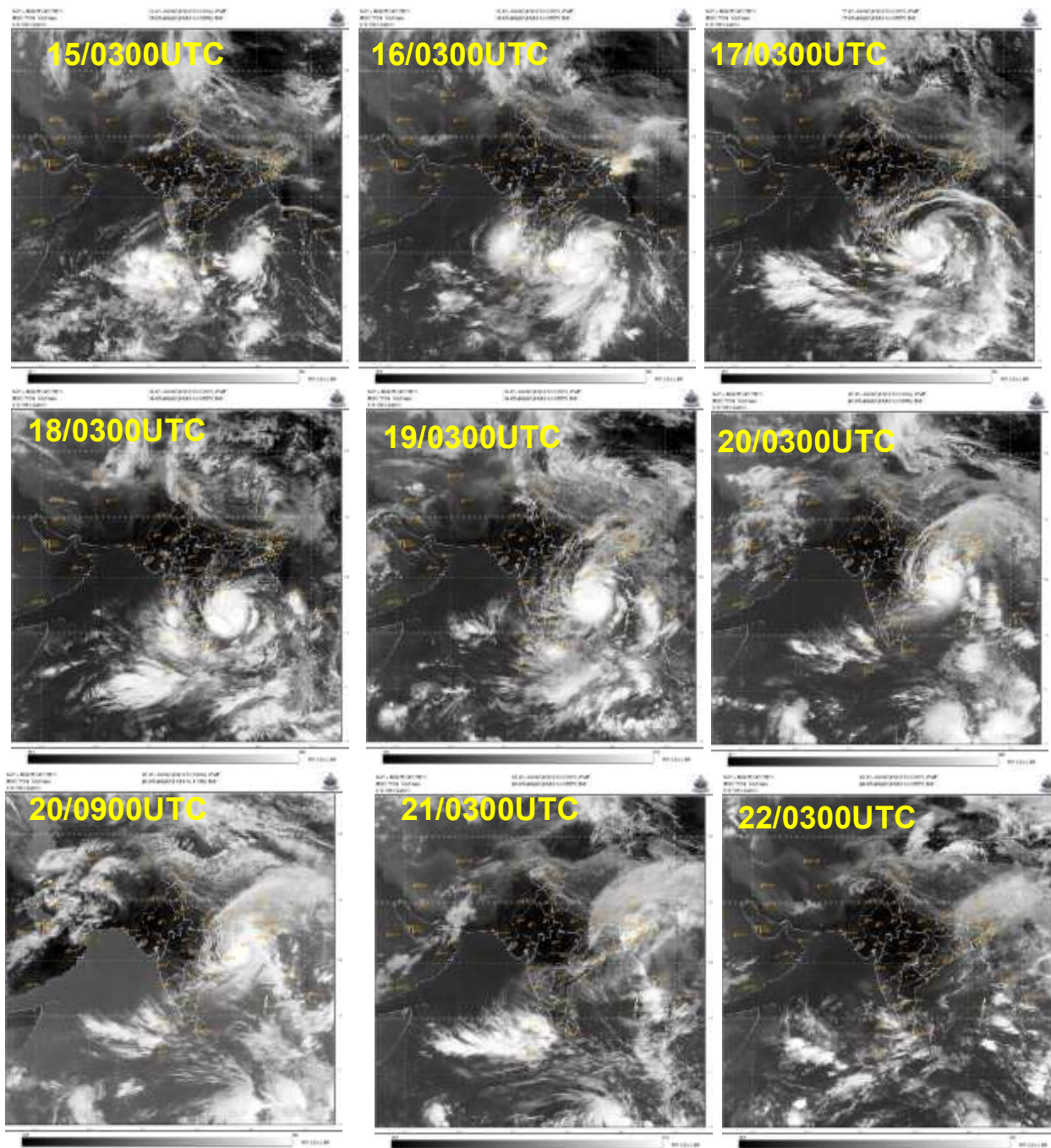
Fig. 4: INSAT-3D IR imageries during life cycle of SuCS AMPHAN (15-22 May, 2020)
