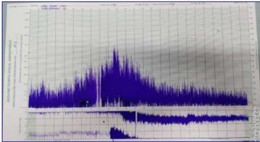
Fig.7: Wind anemograph recordings at Kolkata (Alipore) on 20 th May 2020
