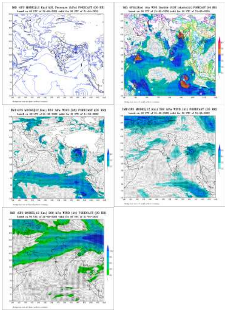
Fig. 14 (i): IMD GFS (T574) mean sea level pressure (MSLP), winds at 10m, 850, 500 and 200 hPa levels based on 0000 UTC of 21 st May,2020
